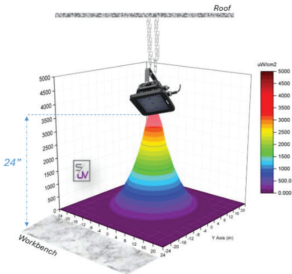
Intensity and coverage area for EDG-13HC at 2 ft (24")
