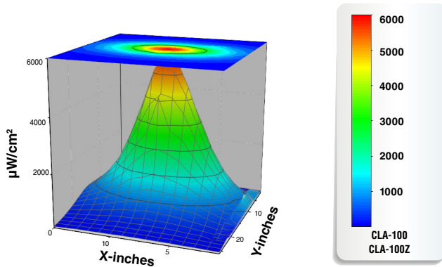
Surface Contour Profile at 15 in (38 cm)
